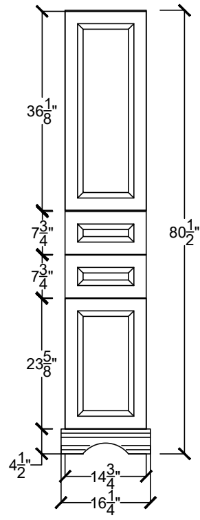
H-ARTTC 1522-2D- - -
