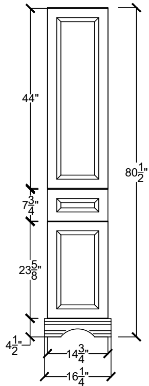
H-ARTTC 1522-1D- - -
