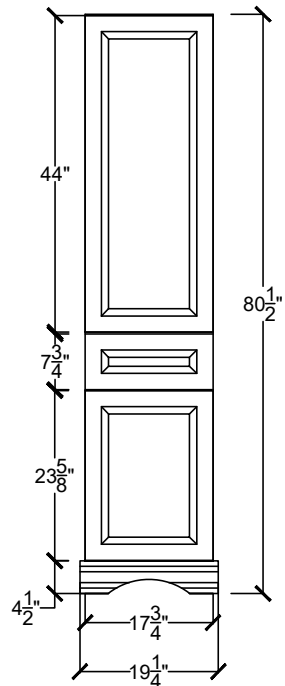
H-ARTTC 1822-1D- - -
