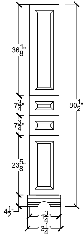
H-ARTTC 1222-2D- _____ - _____ - _____
